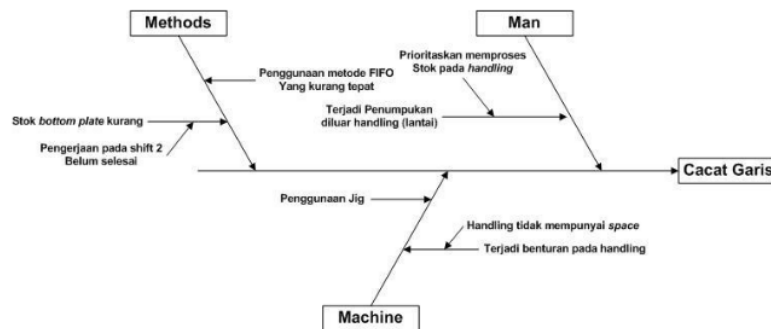
Gambar 7. Fishbone diagram
